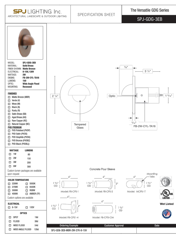
RECESSED WALL LIGHT
